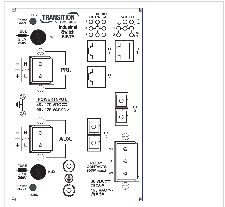
Figure 2: SIBTF10xx-130-MR Front Panel
